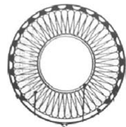
Pipe with thermal insulation and TEMAFOIL™ in between
